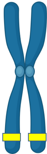
Chromosome B
