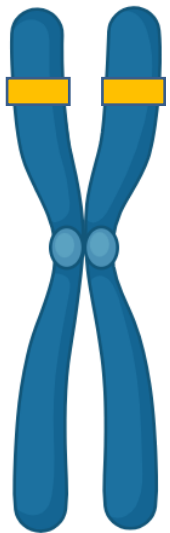
Chromosome A
